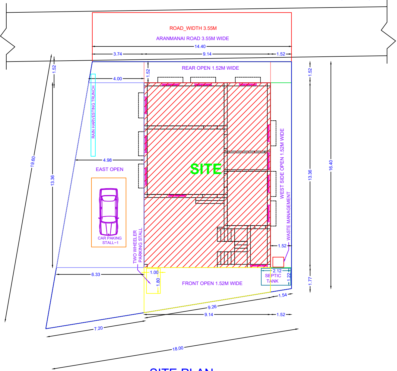
SITE PLAN
