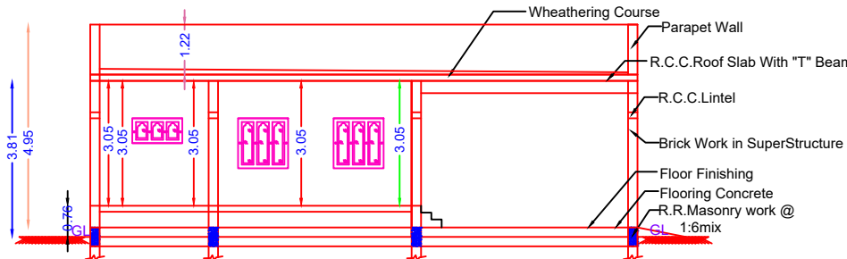
SECTION ON "PQ"
