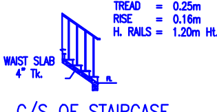
C/S OF STAIRCASE
