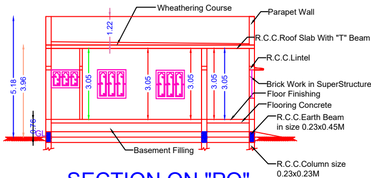
SECTION ON "PQ"
