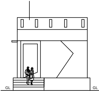
NORTH FACE ELEVATION
