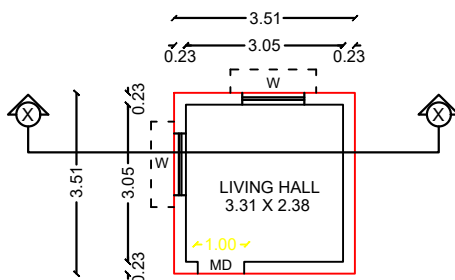
PROPOSED GROUND FLOOR PLAN
