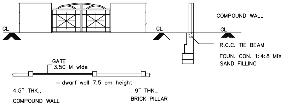
COMPOUND WALL PLAN
