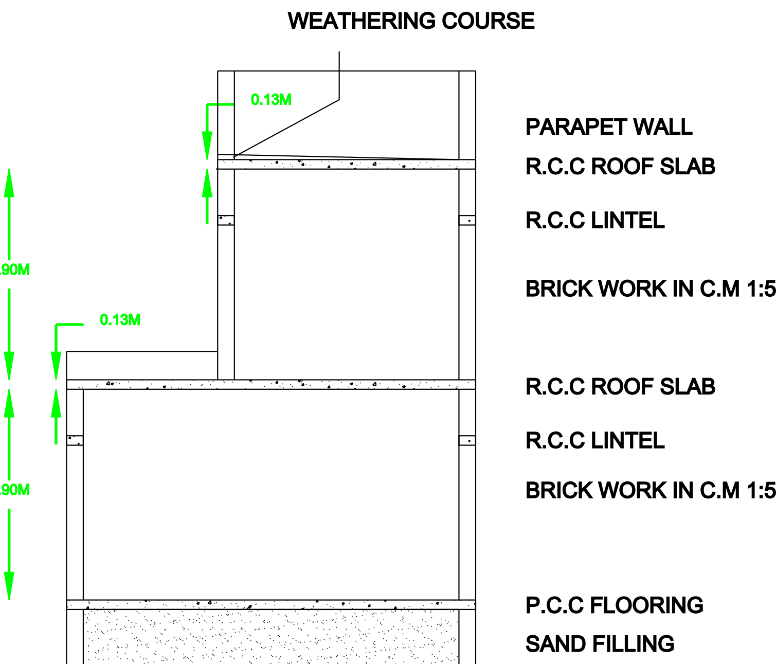
SECTION ON ABCD
