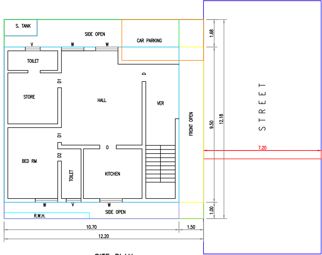
SITE PLAN
