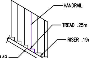
STAIR DETAIL
