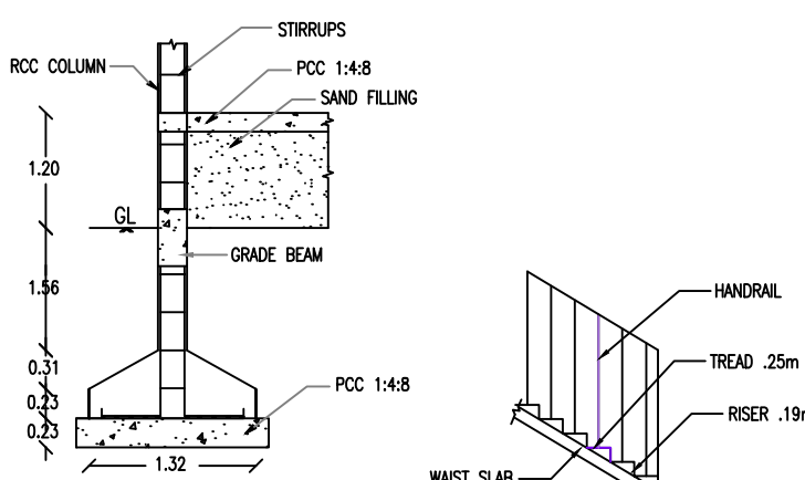
COLUMN DETAILS
