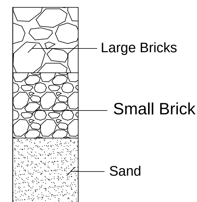
SECTION OF RAIN WATER COLLECTION PITS (NTS)
