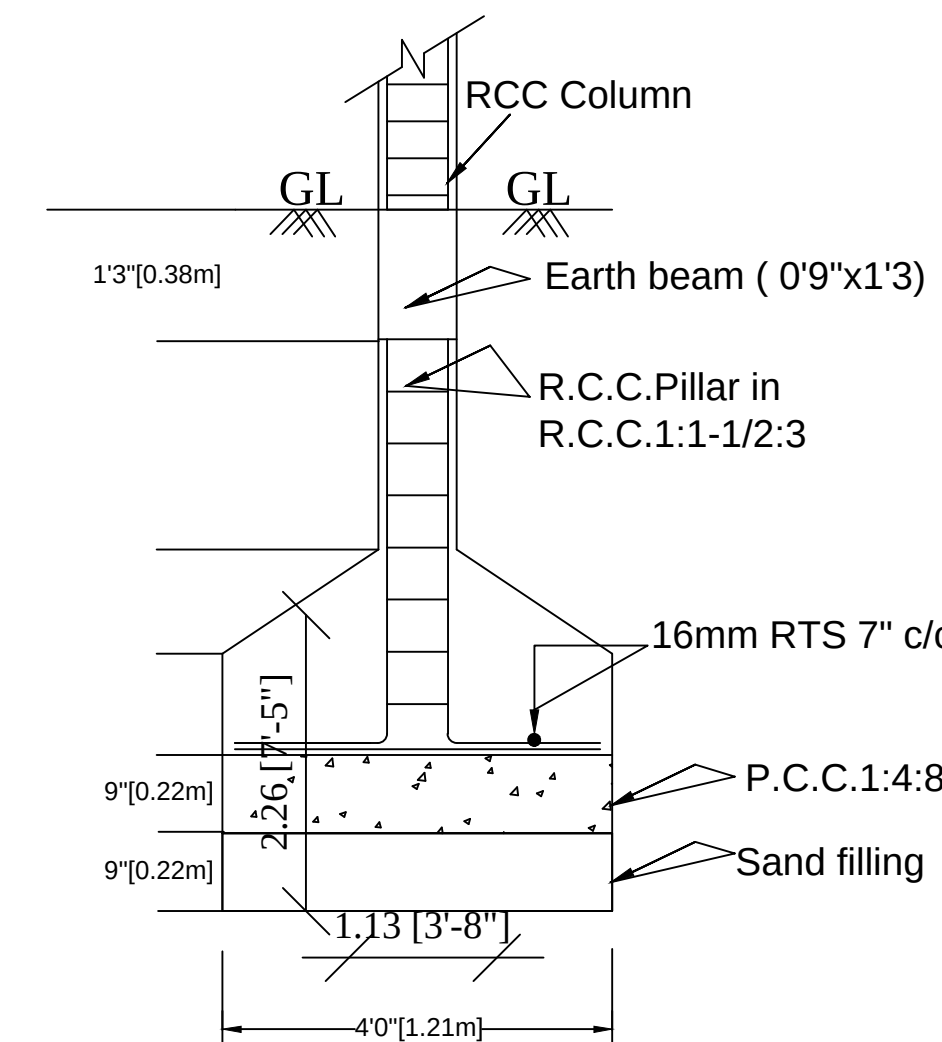
FOUNDATION DETAILS
