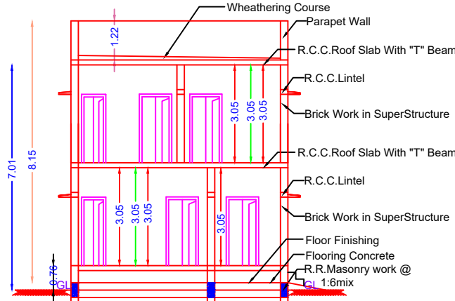
SECTION ON "PQ"
