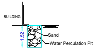
DETAILS OF RAIN WATER PERCOLATION PIT
