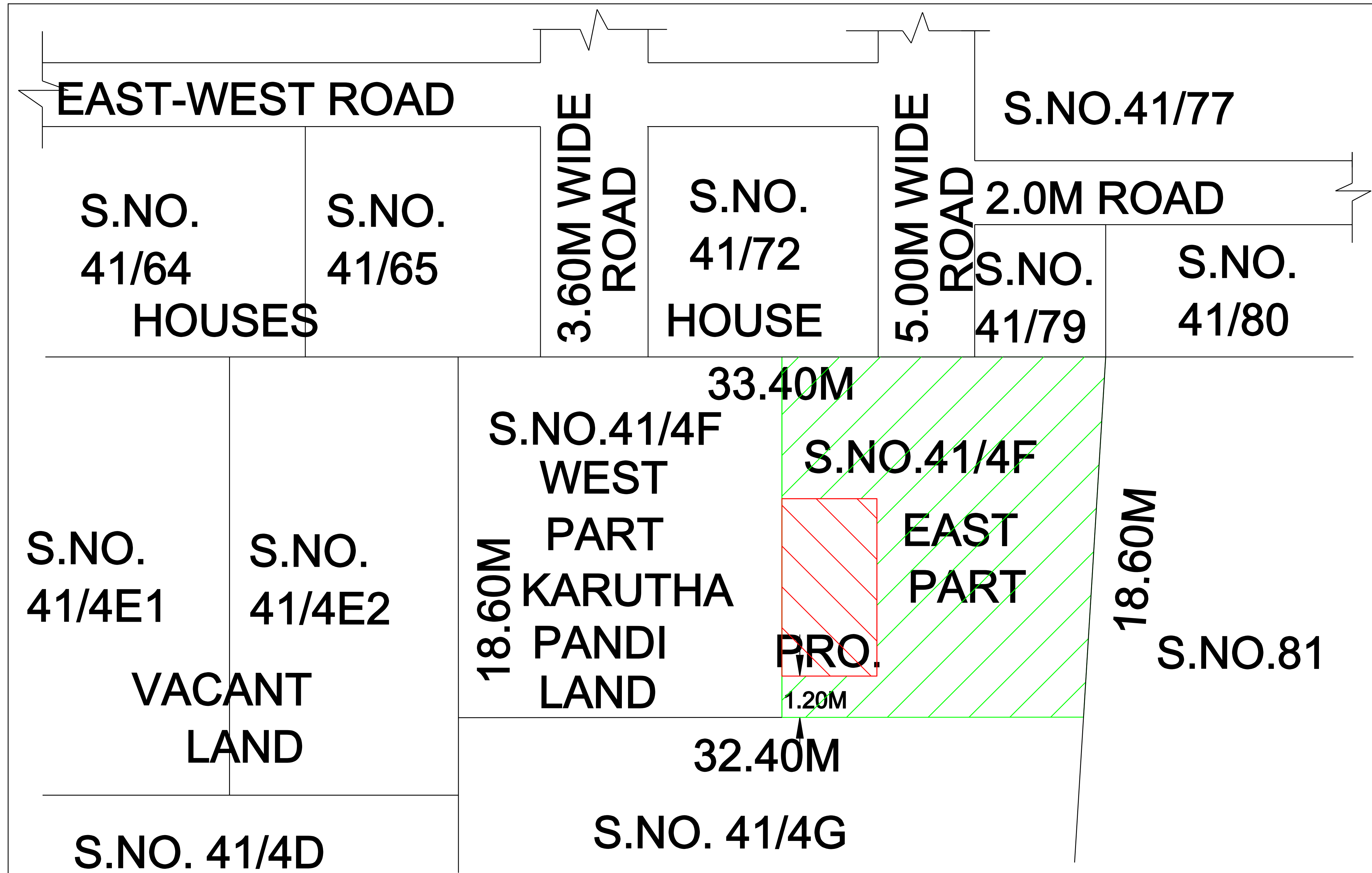
LOCATION PLAN
