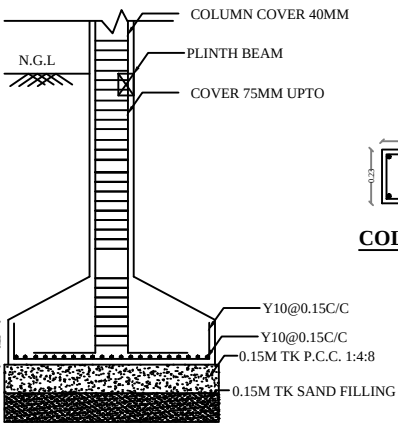
SECTION AT XX
