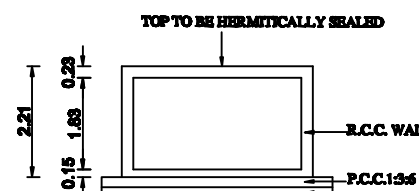
SECTION ON "U.G.SUMP"
