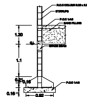
COLUMN DETAIL (SCALE 1:50)
