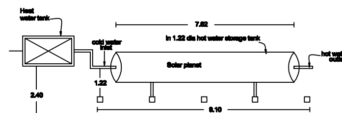
SOLAR WATER HEATER PLANT
