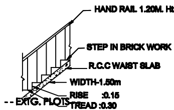
STAIR DETAIL
