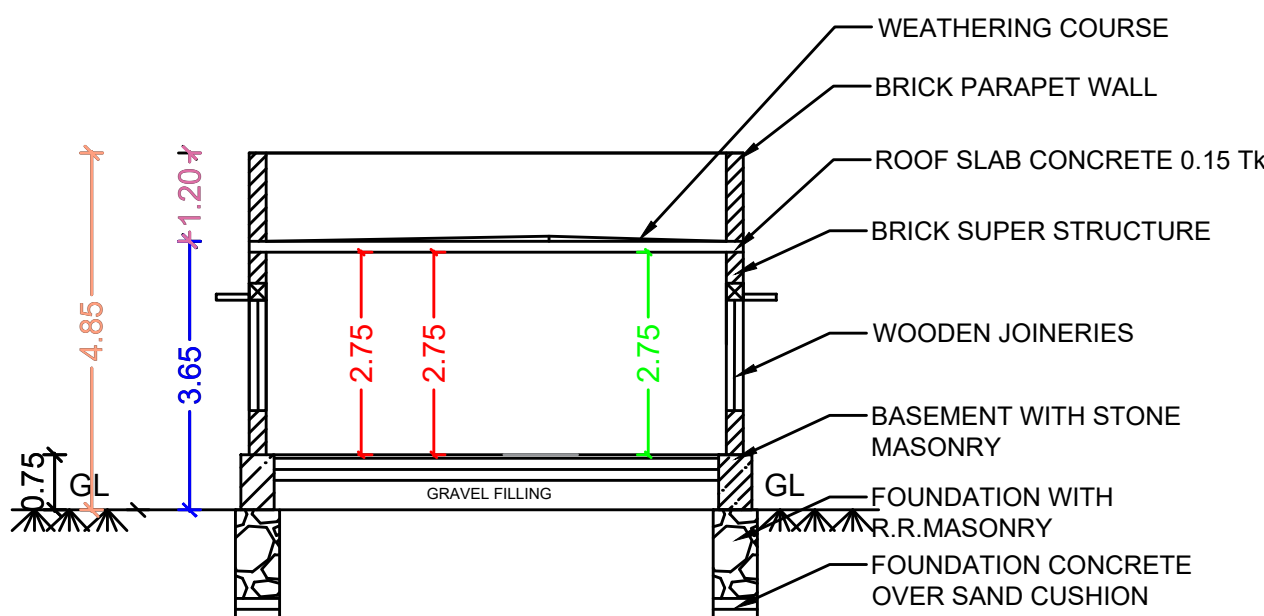
SECTION VIEW"AA"
