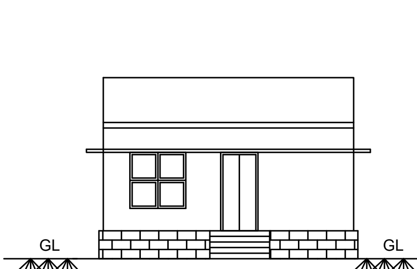
FRONT ELEVATION
