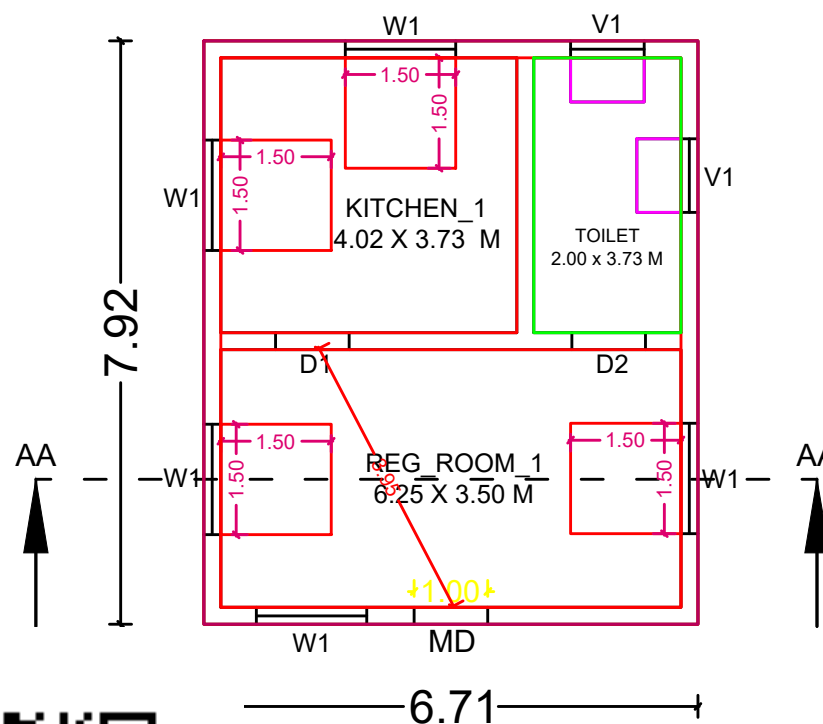
N - GROUND FLOOR (NORTH FACING HOUSE)
