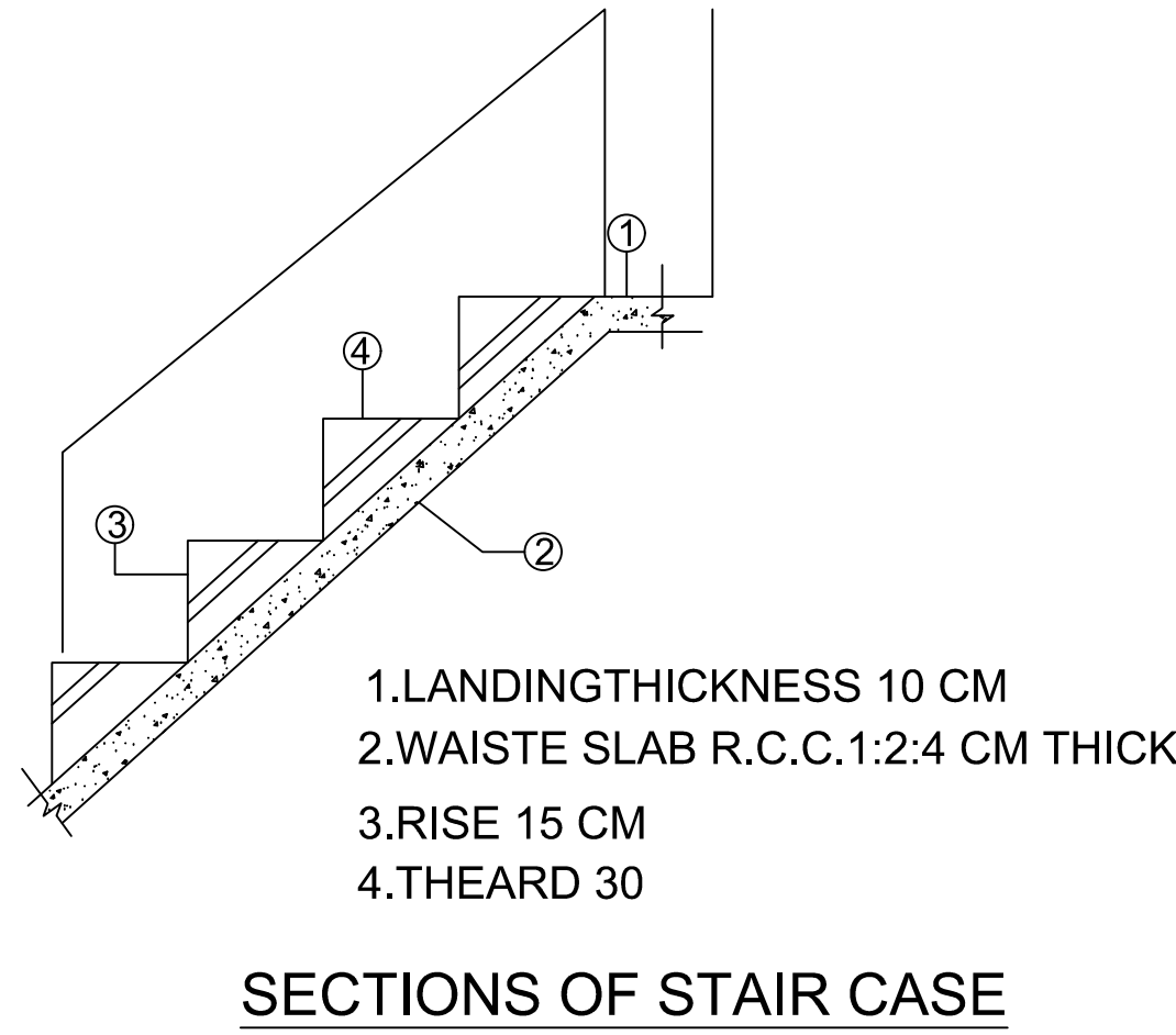
SECTIONS OF STAIR CASE
