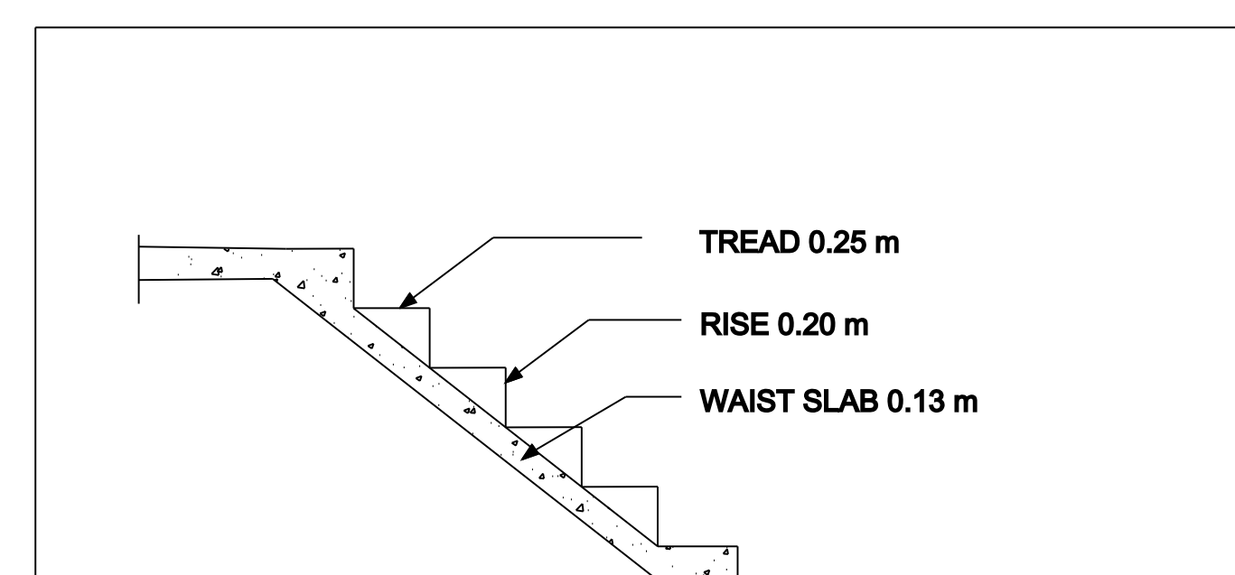
STAIR DETAILS
