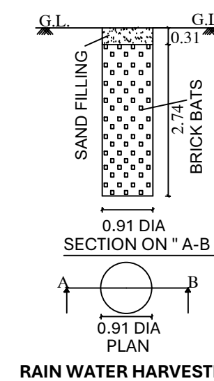
RAIN WATER HARVESTING
