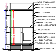
SECTION ON 'XY'
