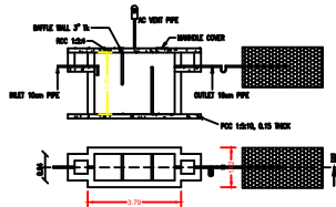
SEPTIC TANK AND TRENCH & U TRAP
