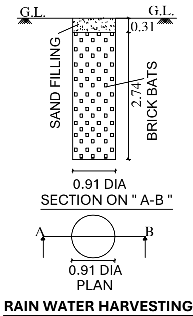
RAIN WATER HARVESTING
