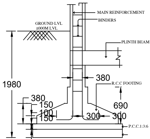
FOUNDATION DETAILS
