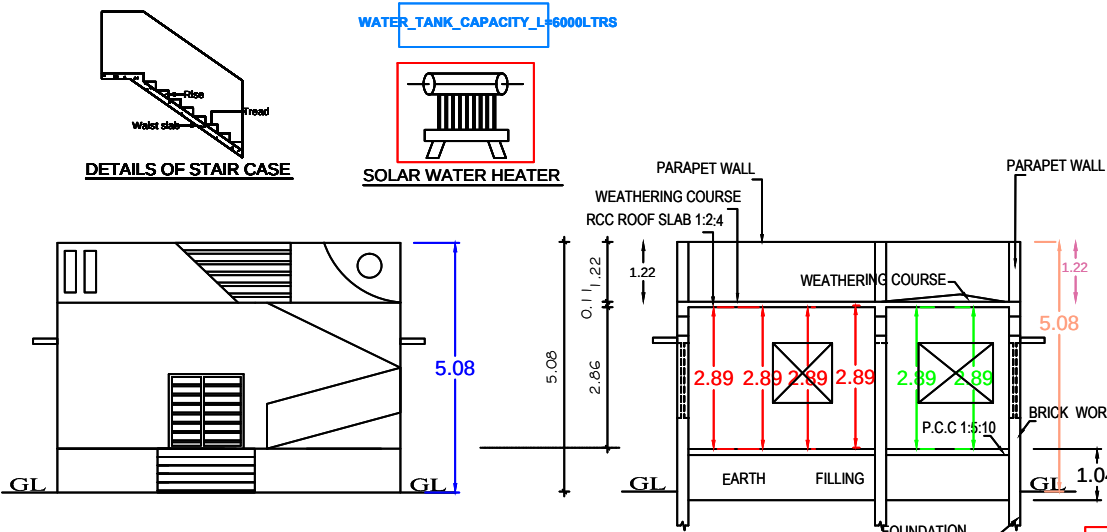
FRONT ELEVATION.
