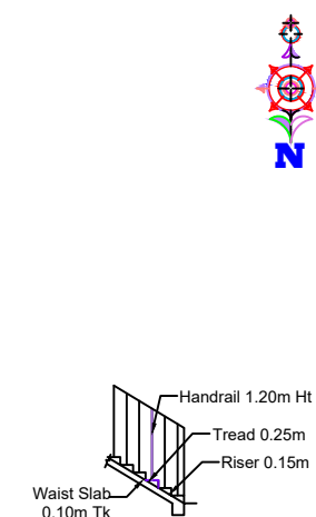
DETAILS OF STAIR CASE (SCALE 1:100)
