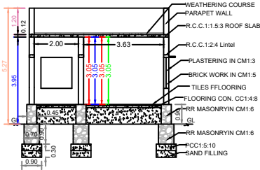
SECTION ON 'XY'
