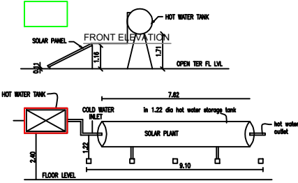
SOLAR WATER HEATER PLANT DETAILS
