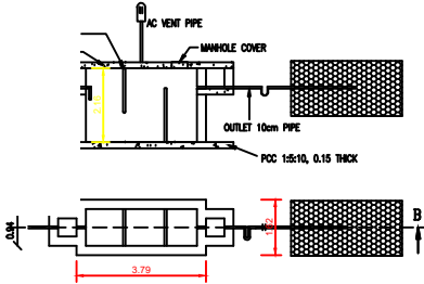
SEPTIC TANK AND TRENCH & U TRAP
