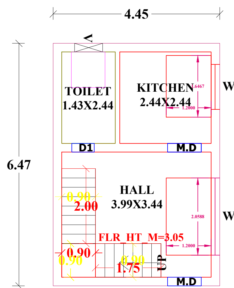
PROPOSED FF PLAN
