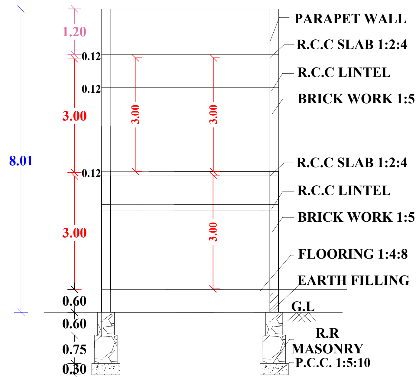
"SECTION "AB"
