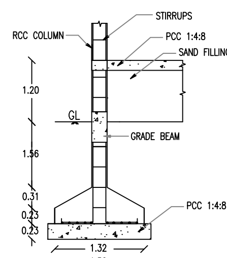
COLUMN DETAILS
