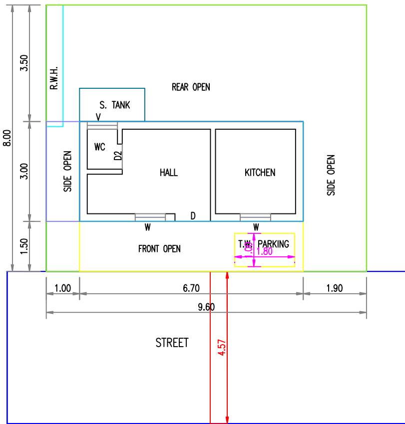
SITE PLAN
