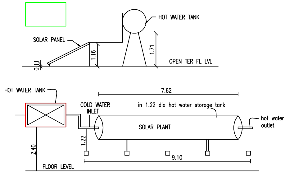
SOLAR WATER HEATER PLANT DETAILS
