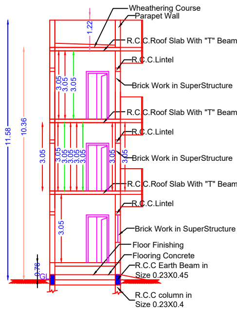
SECTION ON "PQ"
