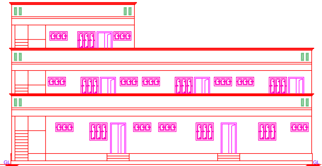
FRONT ELEVATION
