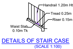
DETAILS OF STAIR CASE (SCALE 1:100)
