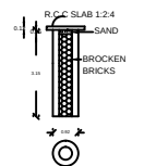
PERCOLATION PIT
