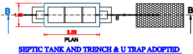
SEPTIC TANK AND TRENCH & U TRAP ADOPTED
