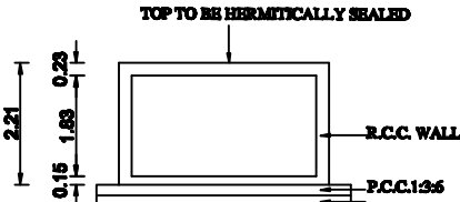
SECTION ON "U.G.SUMP"
