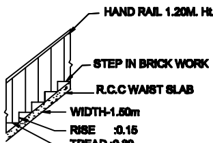
STAIR DETAIL
