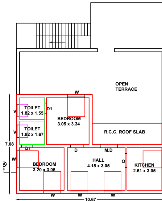
PROPOSED ADDITIONAL FIRST FLOOR PLAN
