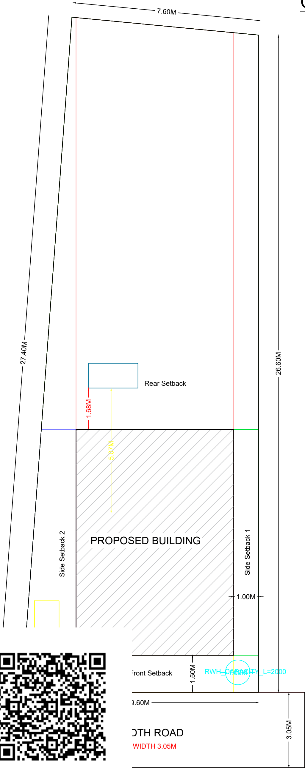
SITE PLAN
