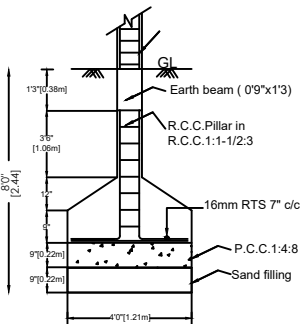
FOUNDATION DETAILS
