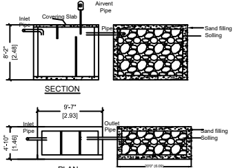
DETAILS OF SEPTIC TANK & DISPERSION TRENCH
