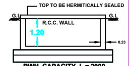
RW SECTION
