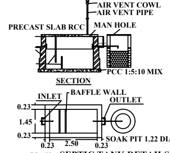
SECTION SEPTIC TANK DETAILS
