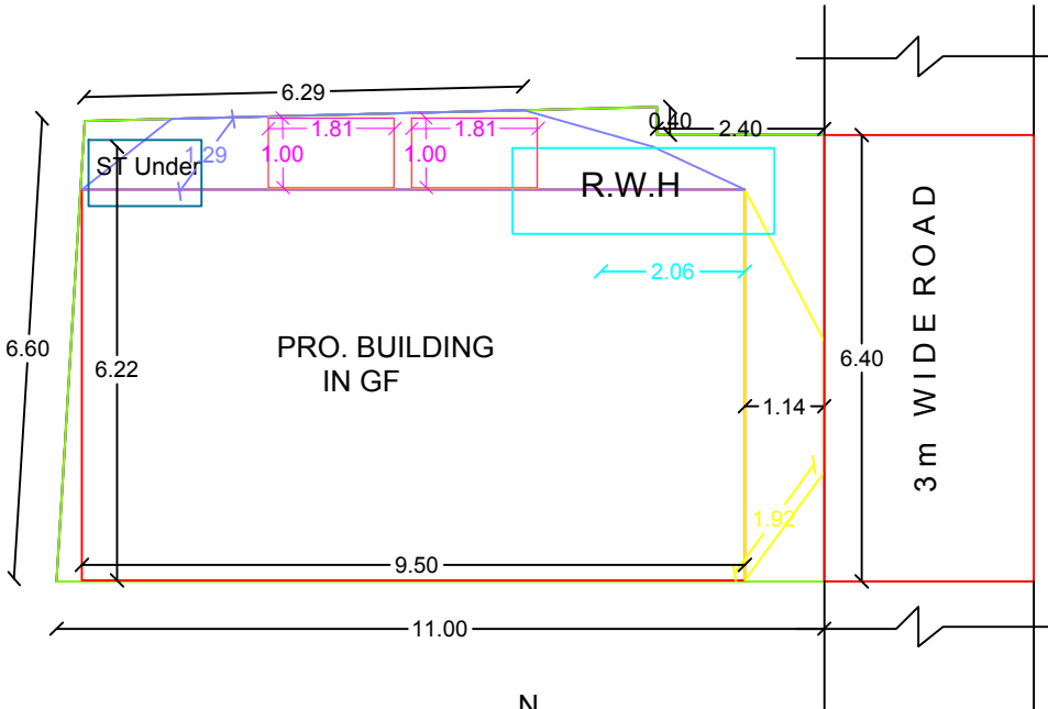
SITE PLAN
