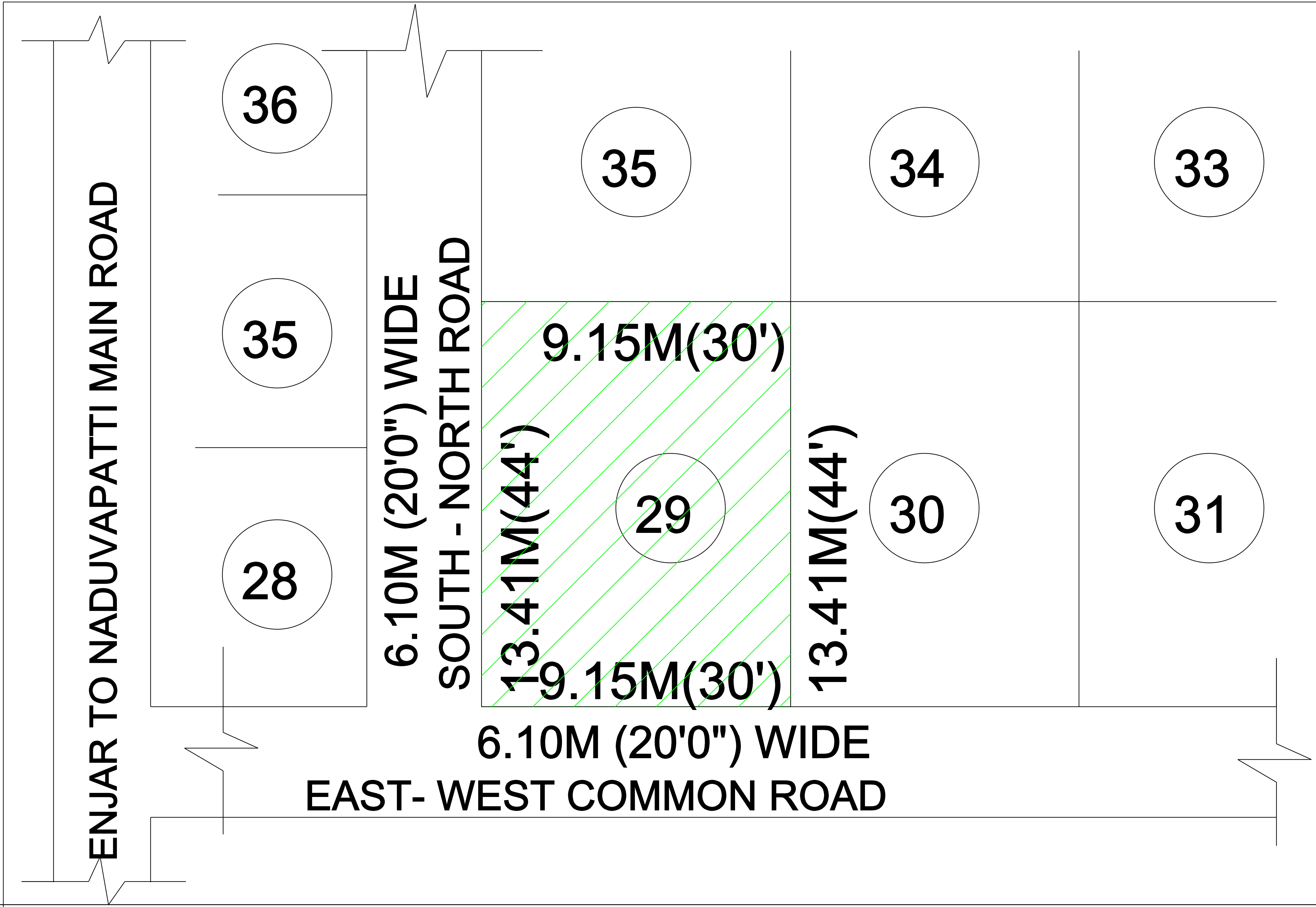
LOCATION PLAN
