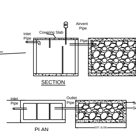
DETAILS OF SEPTIC TANK & DISPERSION TRENCH
