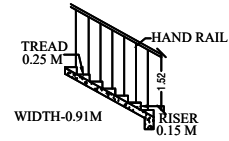
STAIRCASE DETAILS
