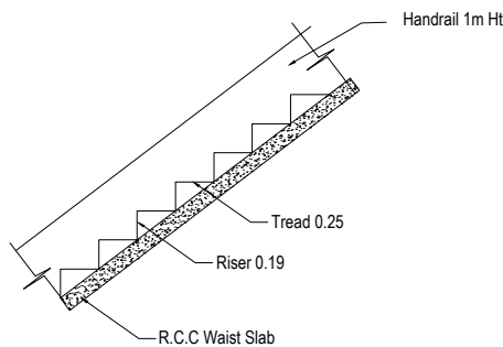
STAIR DETAILS
