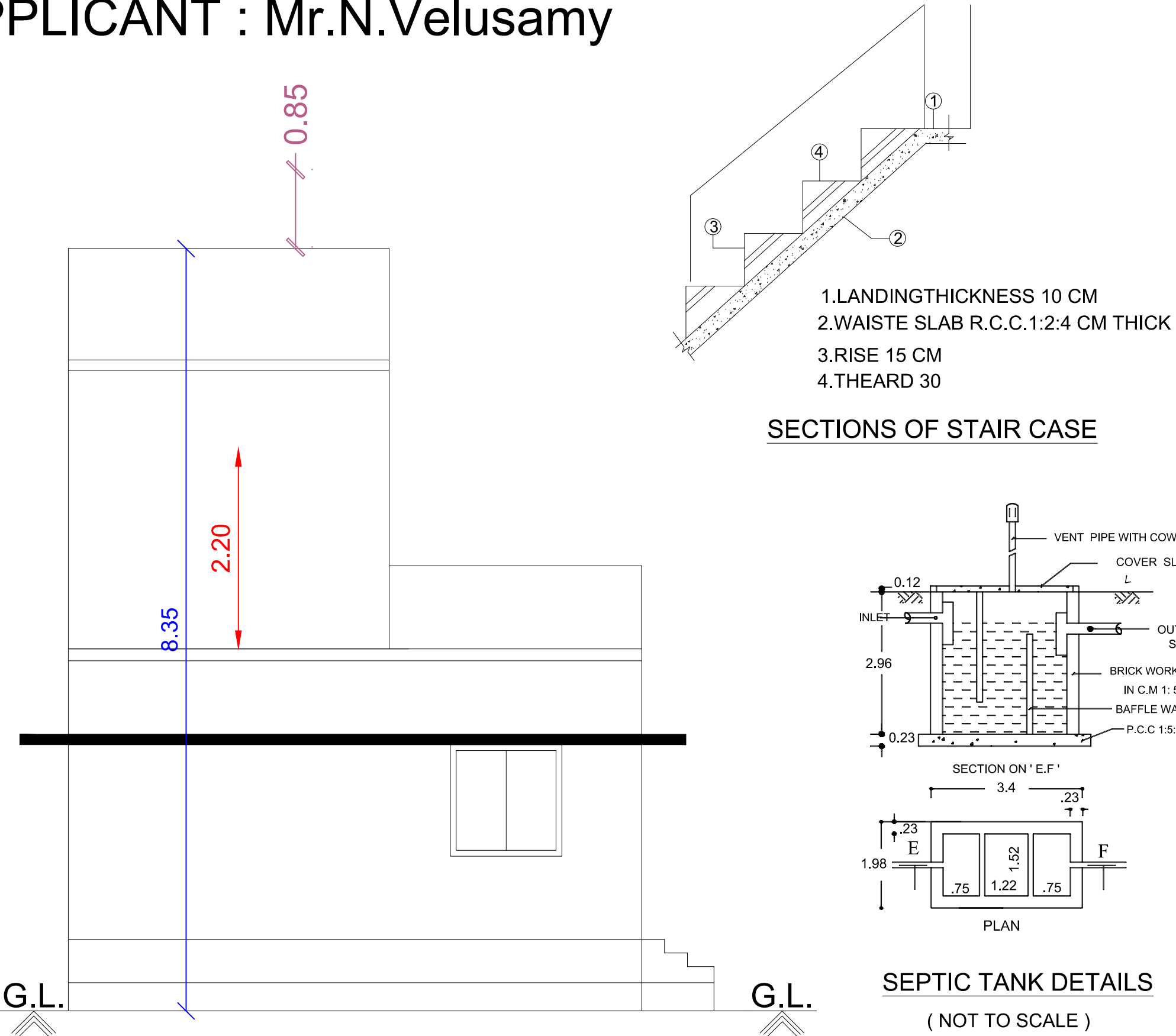
FRONT ELEVATION
