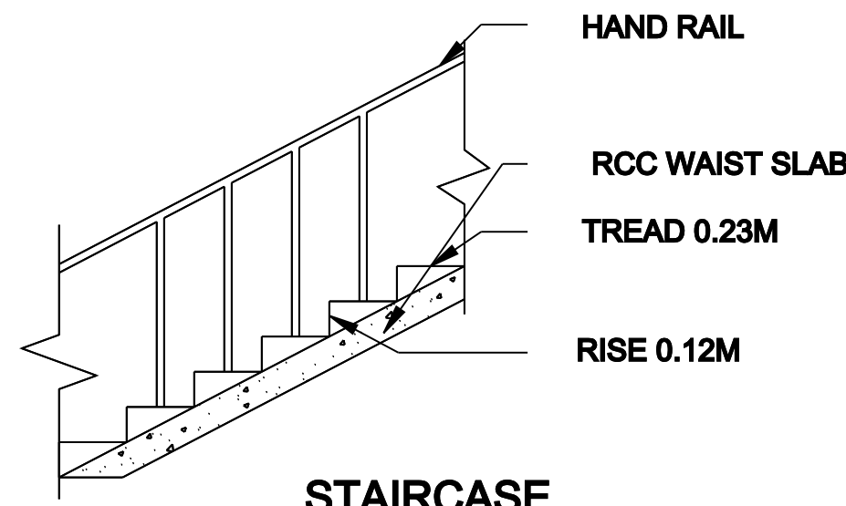
STAIRCASE
