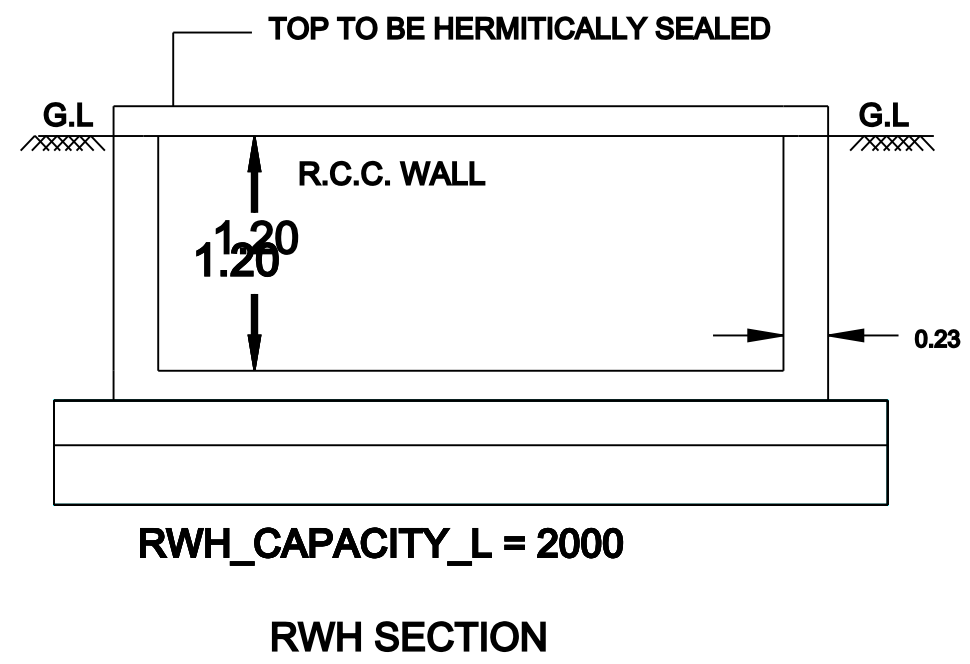
RWHP SECTION
