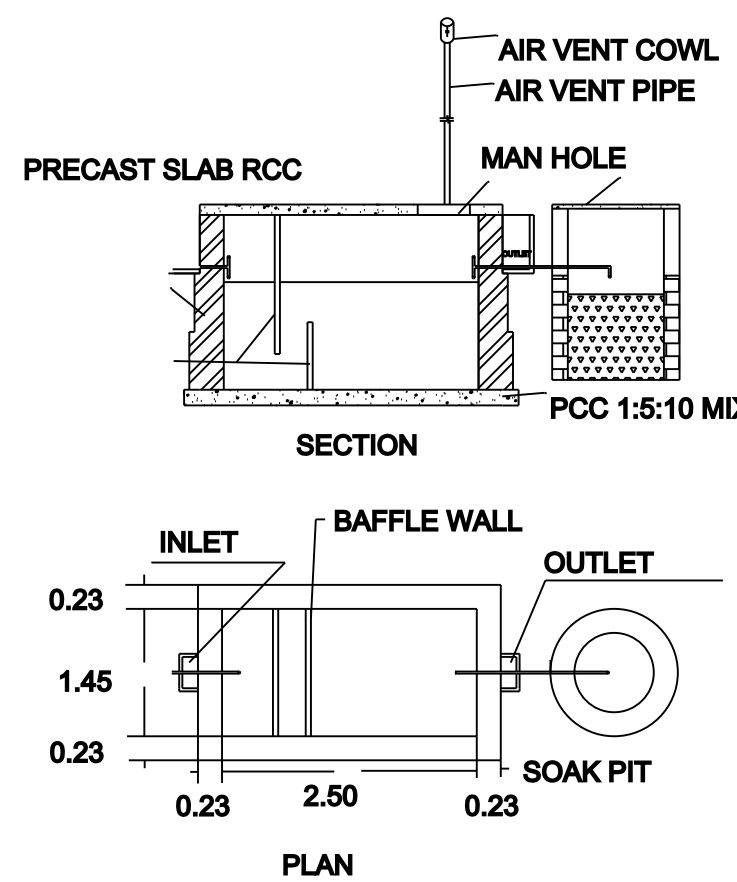
SEPTICTANK DETAILS
