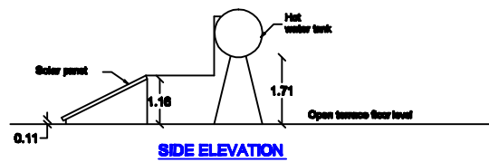
SIDE ELEVATION
