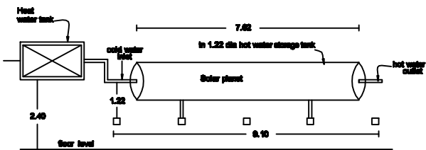
SOLAR WATER HEATER PLANT
