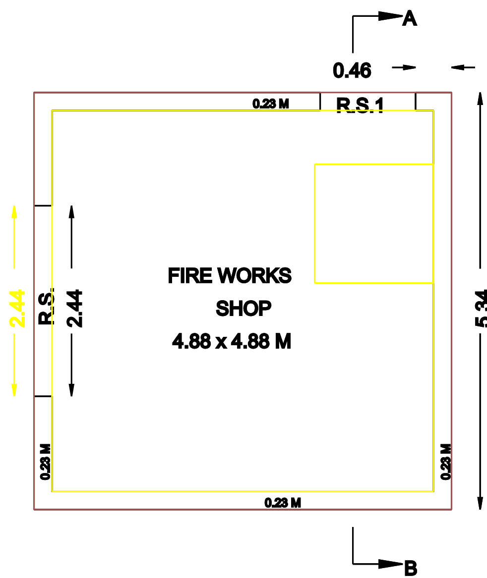
PROPOSED FIRE WORKS SHOP
