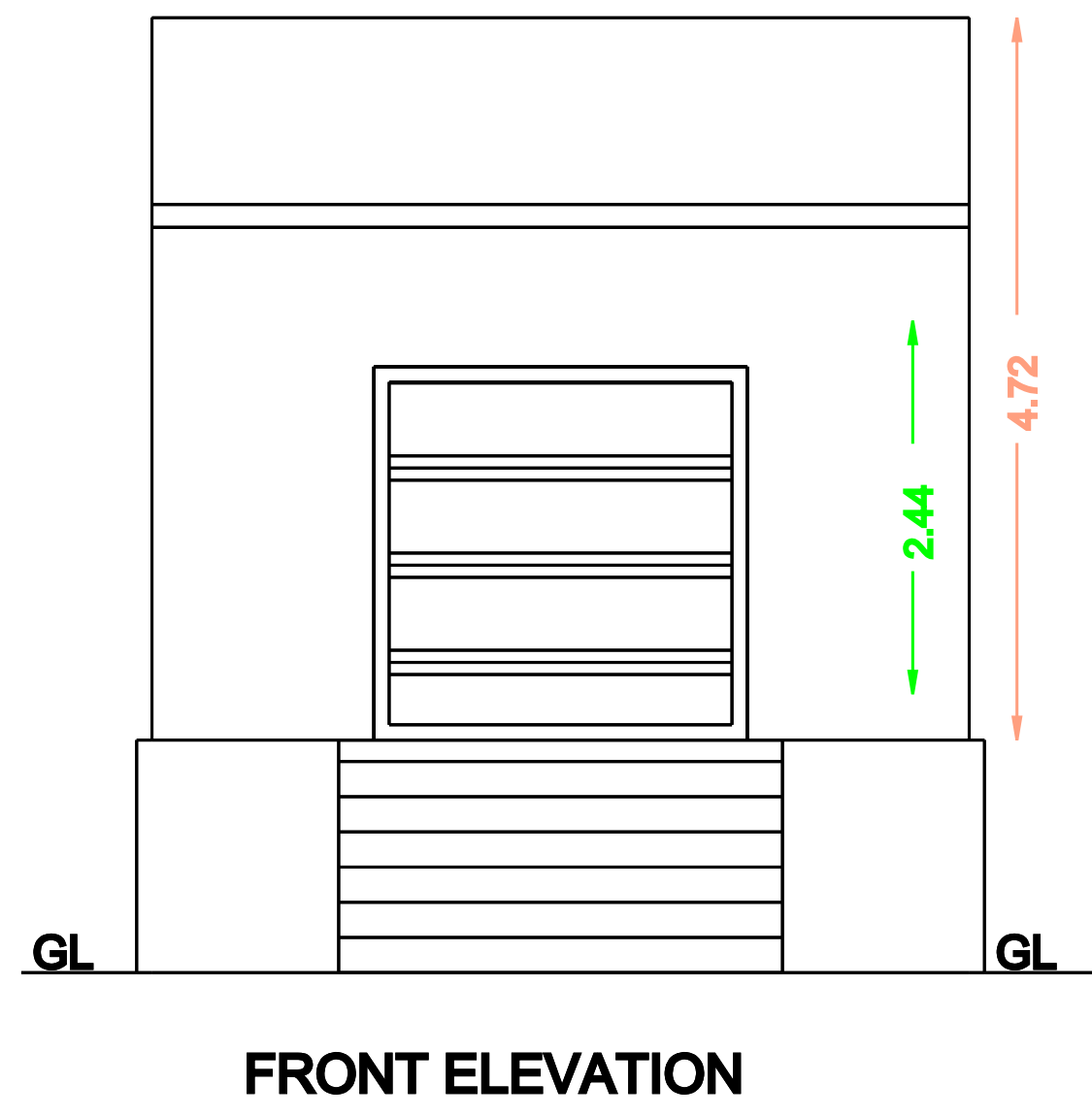
FRONT ELEVATION
