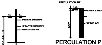
PERCOLATION PIT
