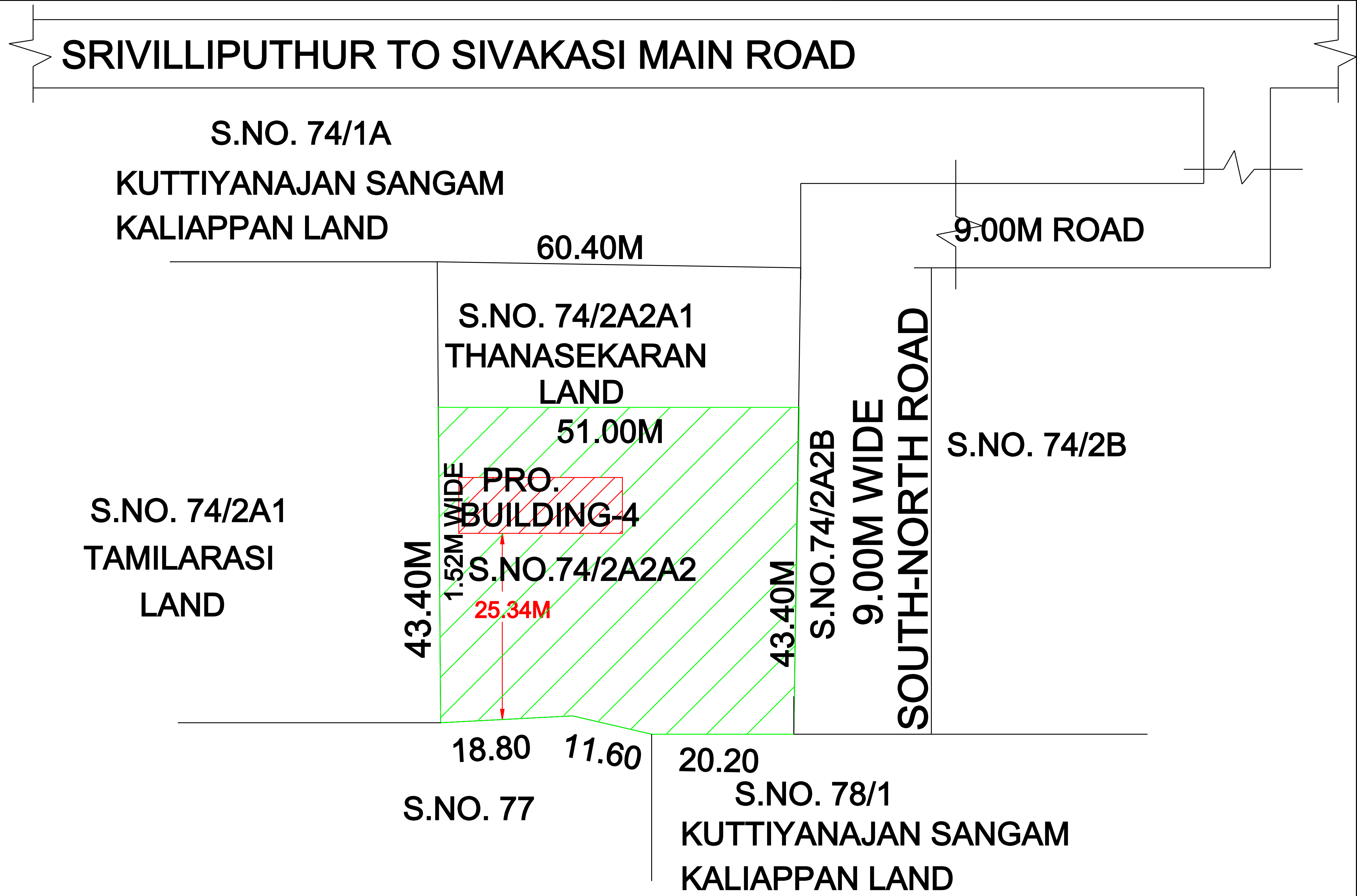
LOCATION PLAN
