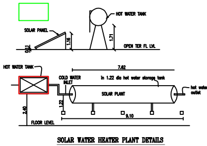
SOLAR WATER HEATER PLANT DETAILS
