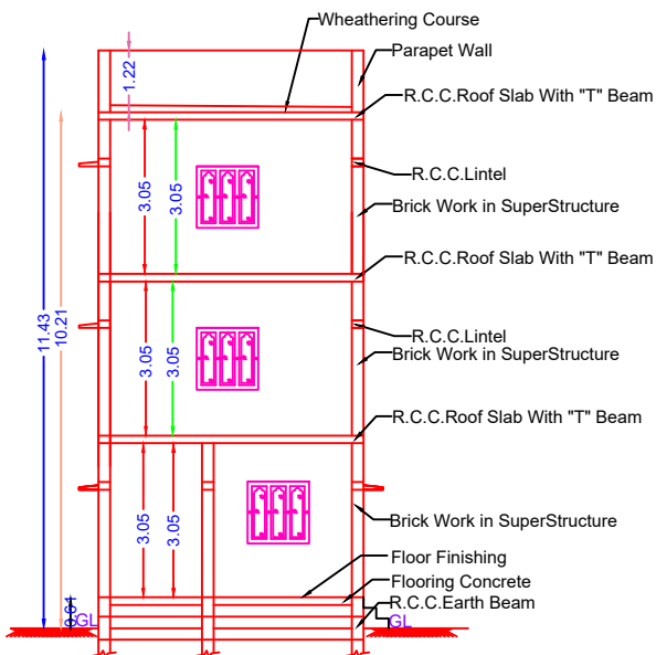
SECTION ON "PQ" SCALE 1:100
