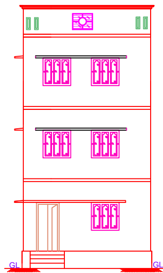
FRONT ELEVATION
