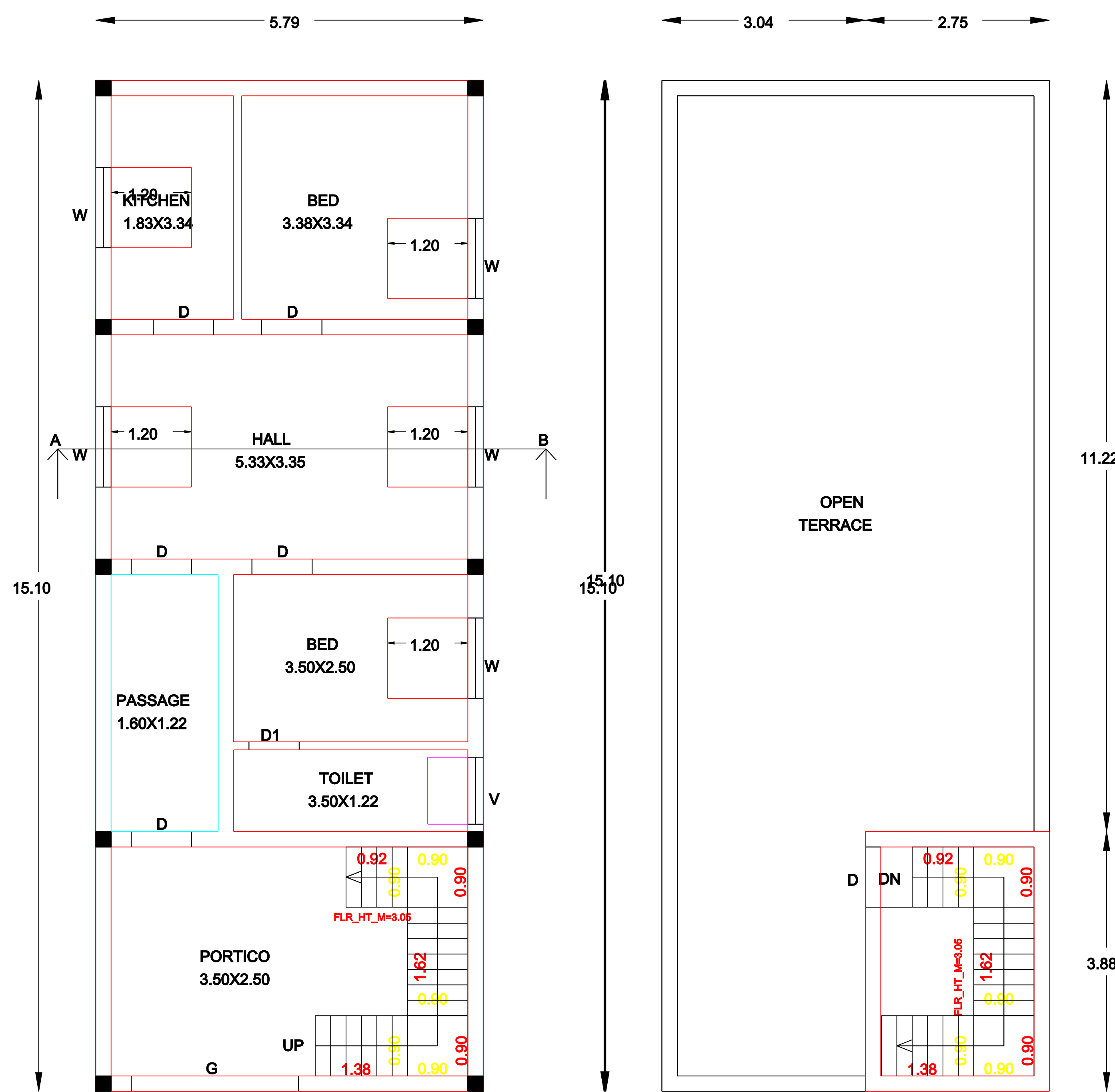
GF PLAN
