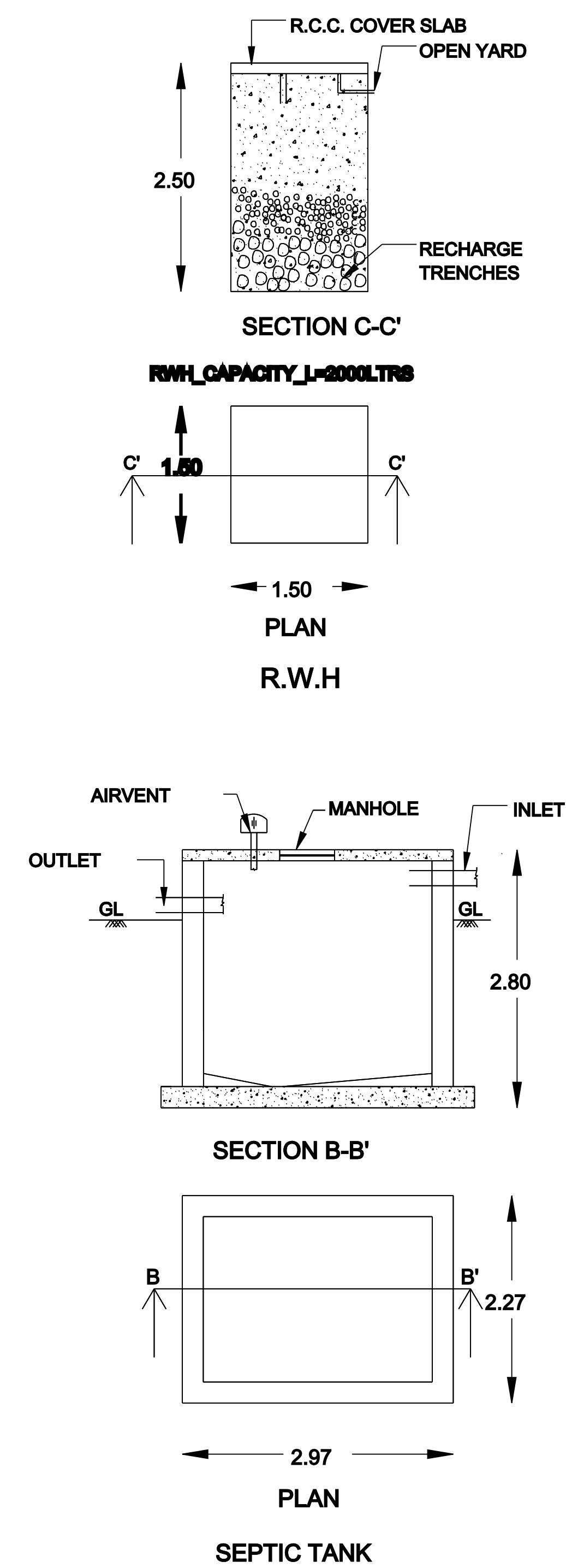
SEPTIC TANK
