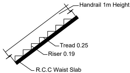
STAIR DETAILS
