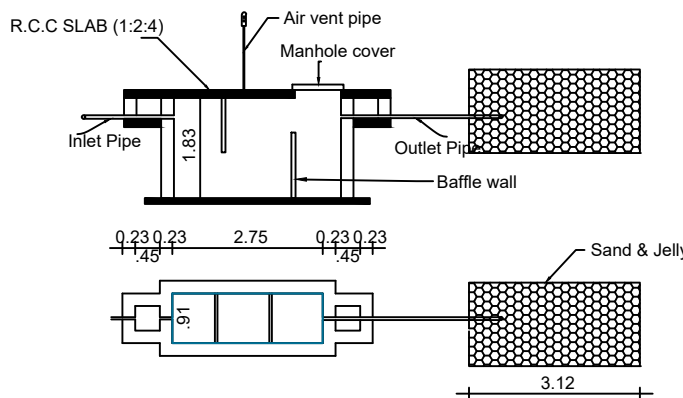
SEPTIC TANK & TRENCH
