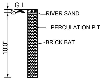
PERCOLATION PIT
