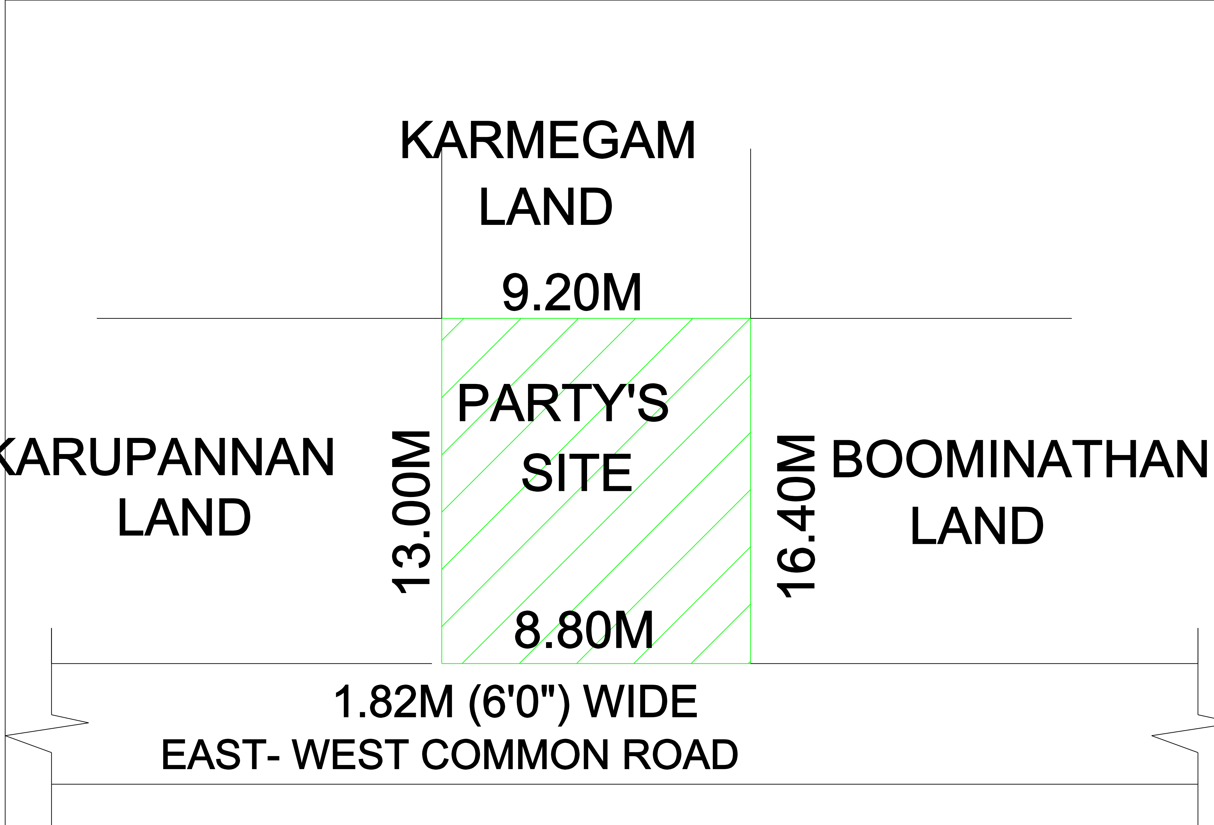
LOCATION PLAN
