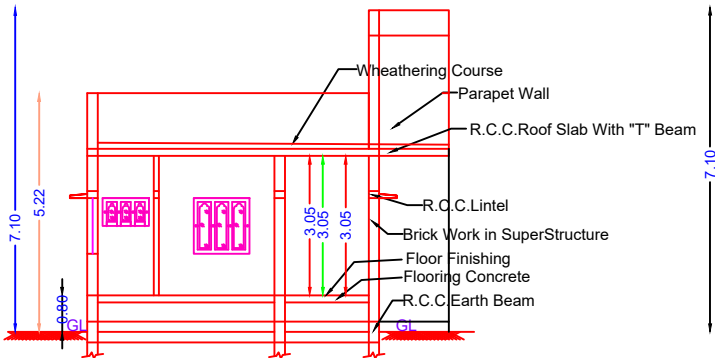
SECTION ON "PQ" SCALE 1:100
